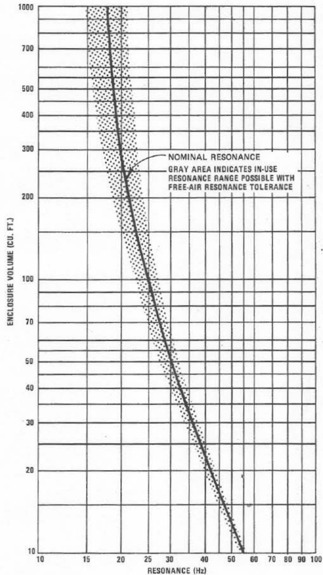
FIGURE 1 — Enclosure Volume vs Resonance
